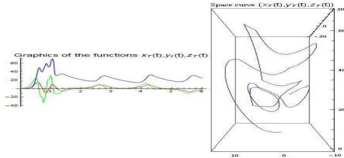
F 3. The solutions x_T(t), y_T(t), z_T(t) where T = 0.125 for the system of differential equations (7) of the time interval [0, 6]
