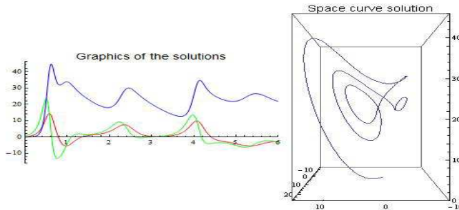
F 1. Results obtained by the program Mathematica for the system (1) of time interval [0, 6]
